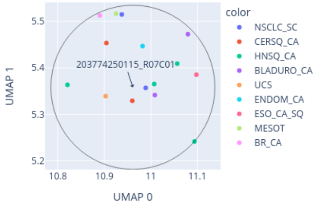
Close-up of UMAP for 203774250115_R07C01 reference: AllIDATv2_20210804_HPAP_Sarc.xlsx (19967 cases), 0 CpGs
