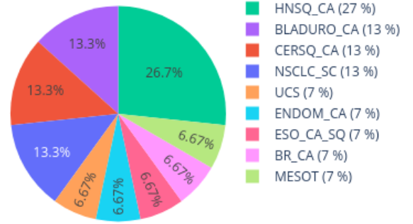
Neighbors in UMAP for 203774250115_R07C01 reference: AllIDATv2_20210804_HPAP_Sarc.xlsx (19967 cases), 0 CpGs
