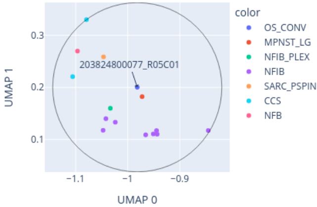
Close-up of UMAP for 203824800077_R05C01 reference: AllIDATv2_20210804_HPAP_Sarc.xlsx (19967 cases), 0 CpGs
