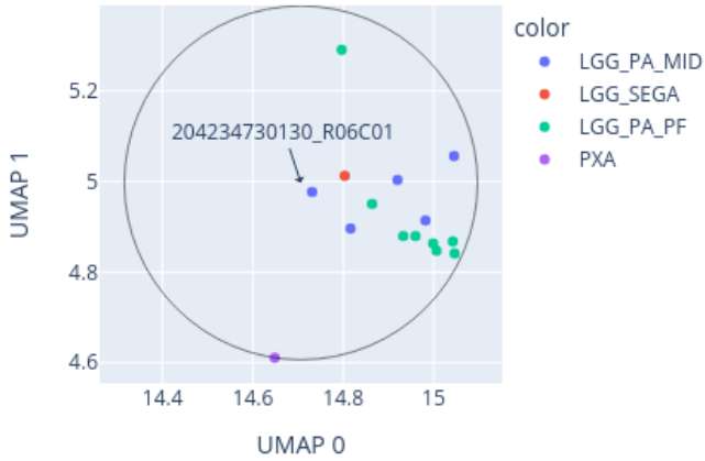
Close-up of UMAP for 204234730130_R06C01 reference: AllIDATv2_20210804_HPAP_Sarc.xlsx (19967 cases), 0 CpGs
