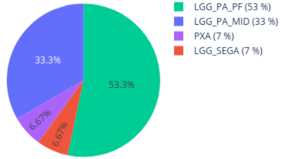
Neighbors in UMAP for 204234730130_R06C01 reference: AllIDATv2_20210804_HPAP_Sarc.xlsx (19967 cases), 0 CpGs
