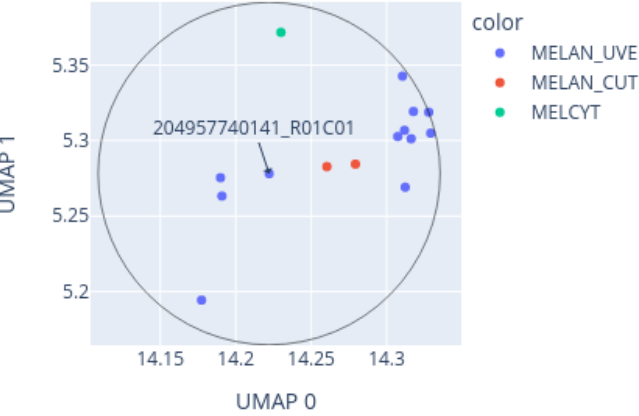
Close-up of UMAP for 204957740141_R01C01 reference: AllIDATv2_20210804_HPAP_Sarc.xlsx (19967 cases), 0 CpGs
