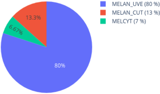
Neighbors in UMAP for 204957740141_R01C01 reference: AllIDATv2_20210804_HPAP_Sarc.xlsx (19967 cases), 0 CpGs
