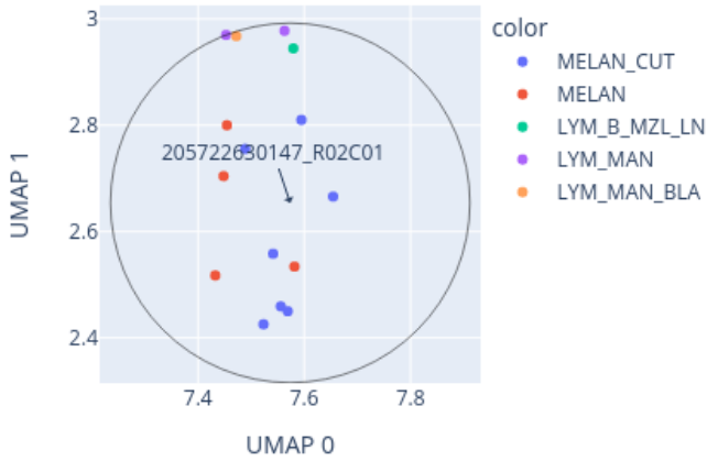
Close-up of UMAP for 205722630147_R02C01 reference: AllIDATv2_20210804_HPAP_Sarc.xlsx (19967 cases), 0 CpGs
