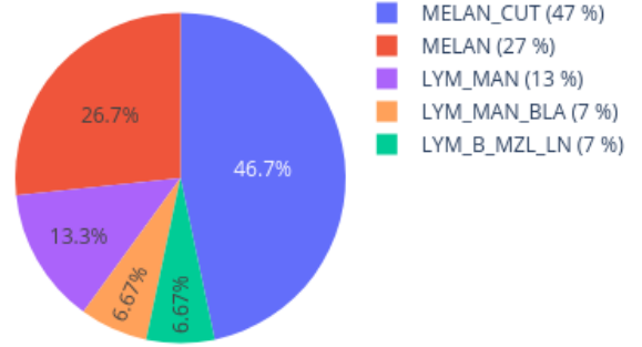
Neighbors in UMAP for 205722630147_R02C01 reference: AllIDATv2_20210804_HPAP_Sarc.xlsx (19967 cases), 0 CpGs
