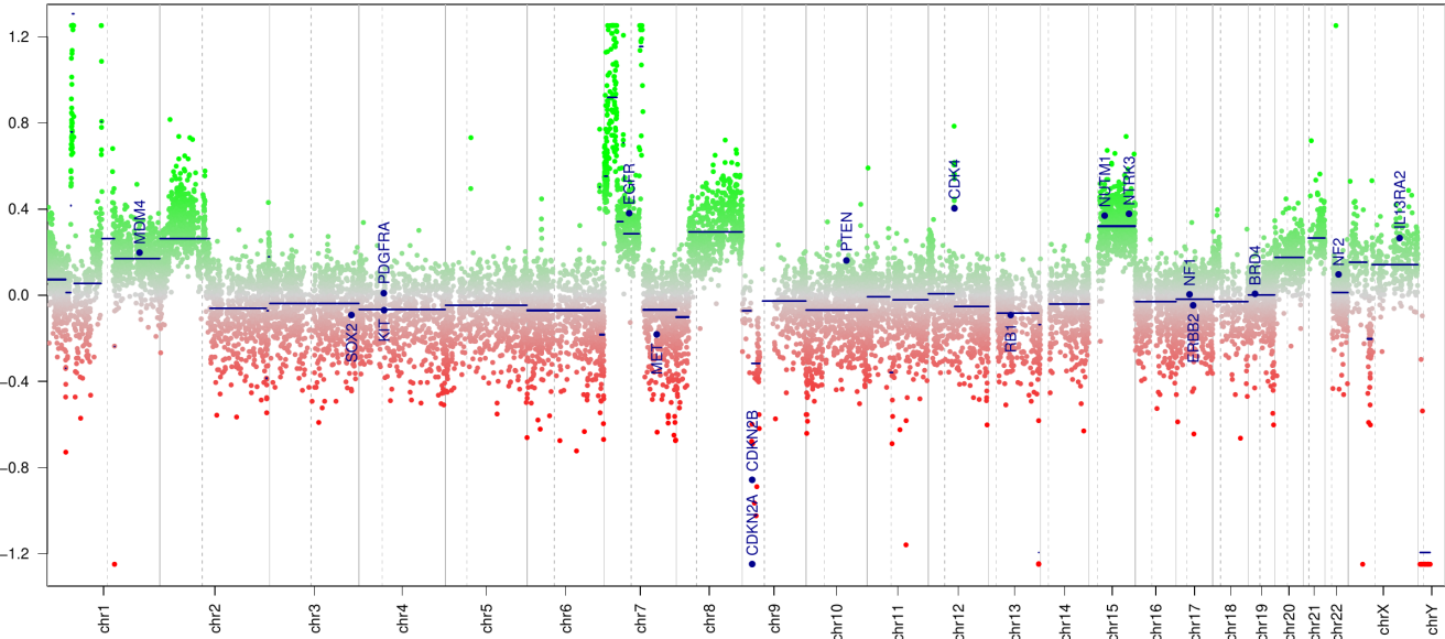
206176580148_R06C01
