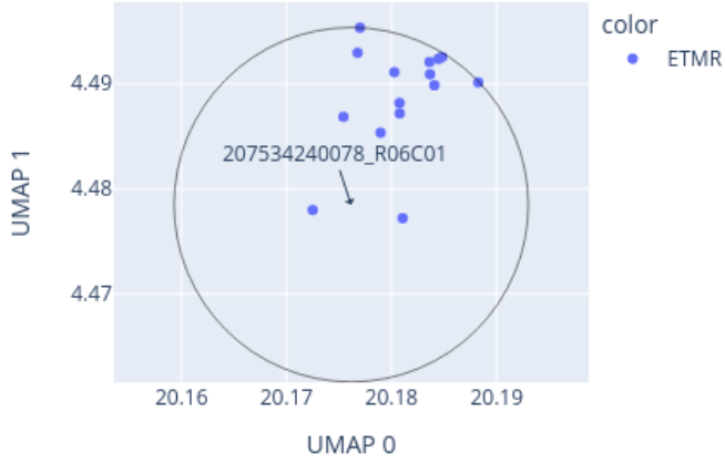
Close-up of UMAP for 207534240078_R06C01 reference: AllIDATv2_20210804_HPAP_Sarc.xlsx (19967 cases), 0 CpGs
