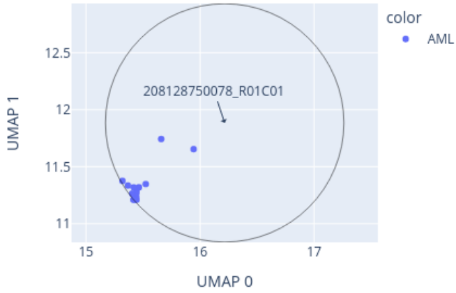
Close-up of UMAP for 208128750078_R01C01 reference: AllIDATv2_20210804_HPAP_Sarc.xlsx (19967 cases), 0 CpGs
