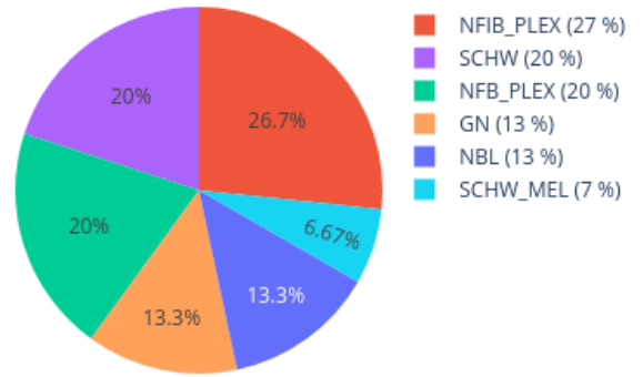
Neighbors in UMAP for 208168230076_R03C01 reference: AllIDATv2_20210804_HPAP_Sarc.xlsx (19967 cases), 0 CpGs
