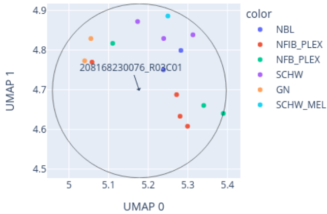
Close-up of UMAP for 208168230076_R03C01 reference: AllIDATv2_20210804_HPAP_Sarc.xlsx (19967 cases), 0 CpGs
