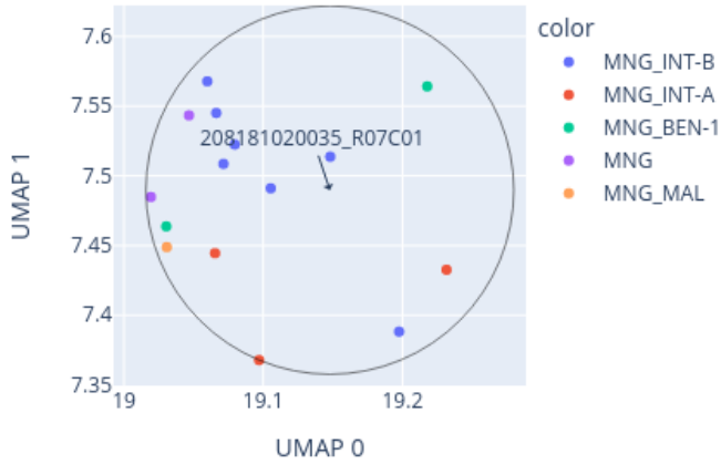
Close-up of UMAP for 208181020035_R07C01 reference: AllIDATv2_20210804_HPAP_Sarc.xlsx (19967 cases), 0 CpGs
