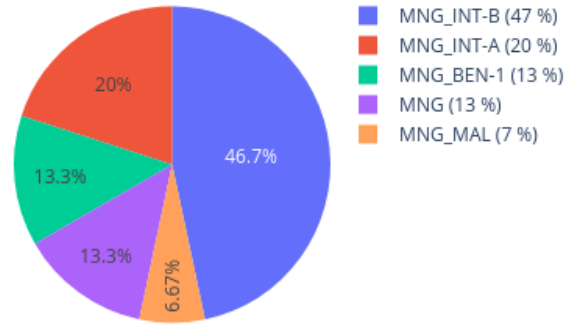
Neighbors in UMAP for 208181020035_R07C01 reference: AllIDATv2_20210804_HPAP_Sarc.xlsx (19967 cases), 0 CpGs
