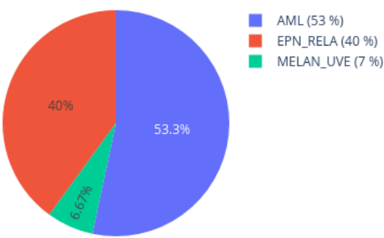
Neighbors in UMAP for 208416840078_R06C01_1 reference: AllIDATv2_20210804_HPAP_Sarc.xlsx (19967 cases), 0 CpGs
