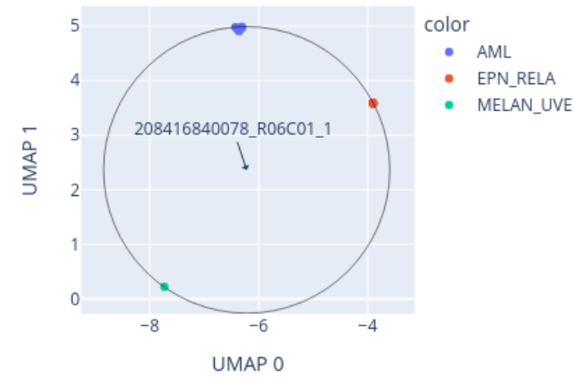
Close-up of UMAP for 208416840078_R06C01_1 reference: AllIDATv2_20210804_HPAP_Sarc.xlsx (19967 cases), 0 CpGs
