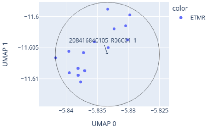
Close-up of UMAP for 208416840105_R06C01_1 reference: AllIDATv2_20210804_HPAP_Sarc.xlsx (19967 cases), 0 CpGs
