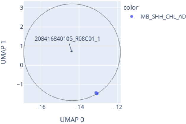
Close-up of UMAP for 208416840105_R08C01_1 reference: AllIDATv2_20210804_HPAP_Sarc.xlsx (19967 cases), 0 CpGs
