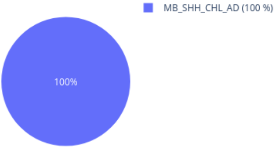
Neighbors in UMAP for 208416840105_R08C01_1 reference: AllIDATv2_20210804_HPAP_Sarc.xlsx (19967 cases), 0 CpGs
