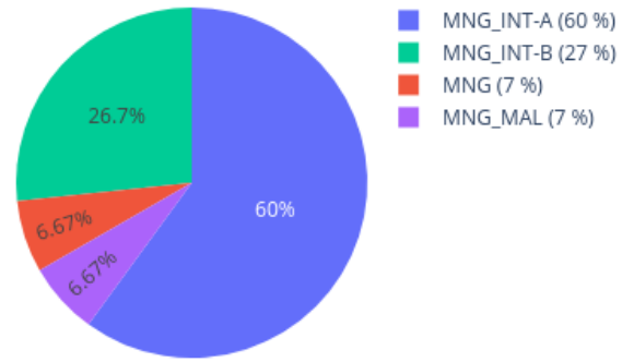
Neighbors in UMAP for 208524750037_R01C01 reference: AllIDATv2_20210804_HPAP_Sarc.xlsx (19967 cases), 0 CpGs
