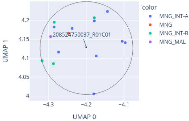
Close-up of UMAP for 208524750037_R01C01 reference: AllIDATv2_20210804_HPAP_Sarc.xlsx (19967 cases), 0 CpGs
