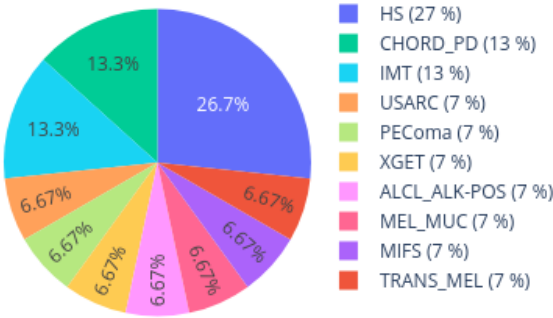
Neighbors in UMAP for 208553420046_R05C01 reference: EpiDip_BTRC_20250105.xlsx (3684 cases), 0 CpGs
