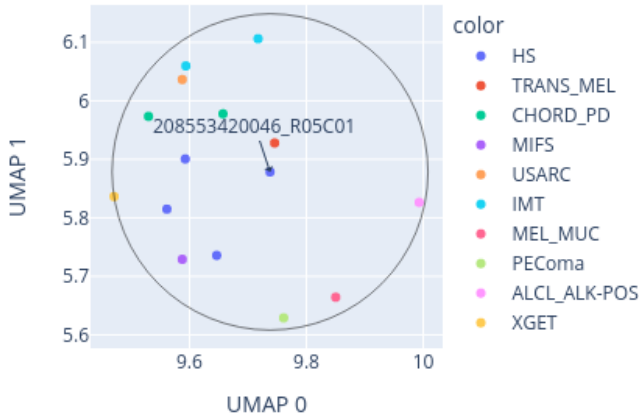
Close-up of UMAP for 208553420046_R05C01 reference: EpiDip_BTRC_20250105.xlsx (3684 cases), 0 CpGs
