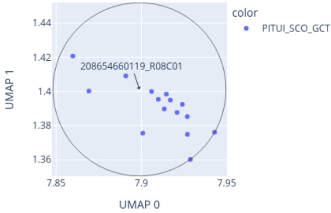
Close-up of UMAP for 208654660119_R08C01 reference: AllIDATv2_20210804_HPAP_Sarc.xlsx (19967 cases), 0 CpGs
