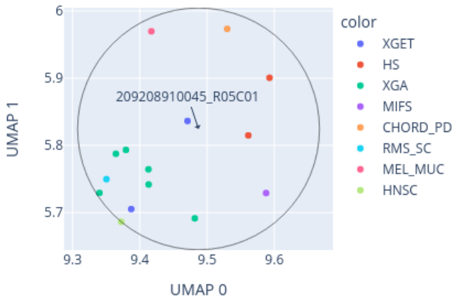
Close-up of UMAP for 209208910045_R05C01 reference: EpiDip_BTRC_20250105.xlsx (3684 cases), 0 CpGs
