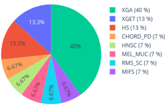
Neighbors in UMAP for 209208910045_R05C01 reference: EpiDip_BTRC_20250105.xlsx (3684 cases), 0 CpGs
