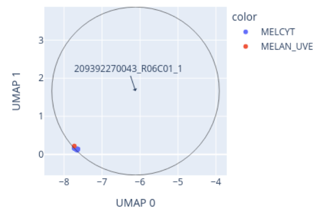
Close-up of UMAP for 209392270043_R06C01_1 reference: AllIDATv2_20210804_HPAP_Sarc.xlsx (19967 cases), 0 CpGs
