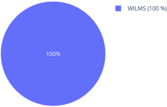
Neighbors in UMAP for 209393000158_R01C01 reference: EpiDip_BTRC_20250105.xlsx (3684 cases), 0 CpGs
