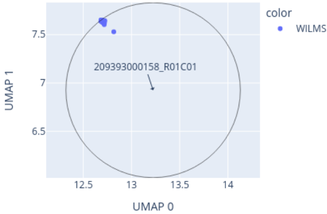
Close-up of UMAP for 209393000158_R01C01 reference: EpiDip_BTRC_20250105.xlsx (3684 cases), 0 CpGs
