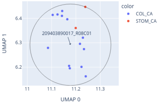
Close-up of UMAP for 209403890017_R08C01 reference: AllIDATv2_20210804_HPAP_Sarc.xlsx (19967 cases), 0 CpGs
