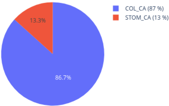
Neighbors in UMAP for 209403890017_R08C01 reference: AllIDATv2_20210804_HPAP_Sarc.xlsx (19967 cases), 0 CpGs
