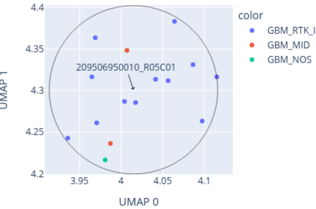
Close-up of UMAP for 209506950010_R05C01 reference: AllIDATv2_20210804_HPAP_Sarc.xlsx (19967 cases), 0 CpGs
