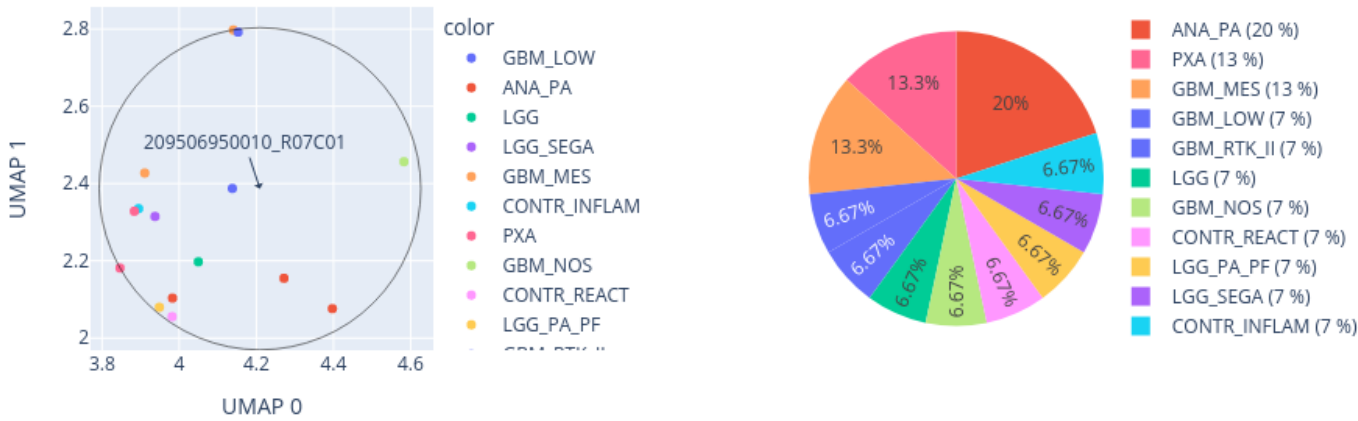
Close-up of UMAP for 209506950010_R07C01 reference: AllIDATv2_20210804_HPAP_Sarc.xlsx (19967 cases), 0 CpGs
