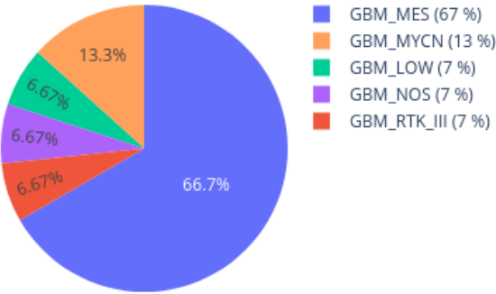
Neighbors in UMAP for 209506950055_R08C01 reference: AllIDATv2_20210804_HPAP_Sarc.xlsx (19967 cases), 0 CpGs
