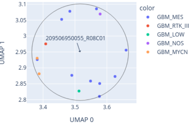
Close-up of UMAP for 209506950055_R08C01 reference: AllIDATv2_20210804_HPAP_Sarc.xlsx (19967 cases), 0 CpGs
