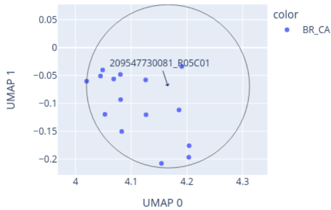
Close-up of UMAP for 209547730081_R05C01 reference: AllIDATv2_20210804_HPAP_Sarc.xlsx (19967 cases), 0 CpGs
