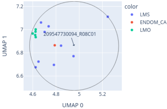
Close-up of UMAP for 209547730094_R08C01 reference: AllIDATv2_20210804_HPAP_Sarc.xlsx (19967 cases), 0 CpGs
