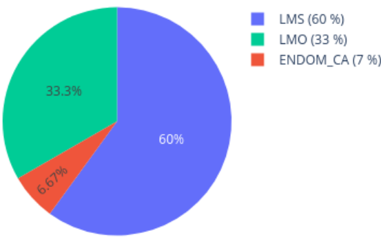
Neighbors in UMAP for 209547730094_R08C01 reference: AllIDATv2_20210804_HPAP_Sarc.xlsx (19967 cases), 0 CpGs
