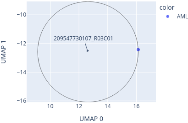
Close-up of UMAP for 209547730107_R03C01 reference: AllIDATv2_20210804_HPAP_Sarc.xlsx (19967 cases), 0 CpGs
