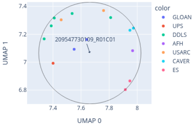
Close-up of UMAP for 209547730109_R01C01 reference: AllIDATv2_20210804_HPAP_Sarc.xlsx (19967 cases), 0 CpGs
