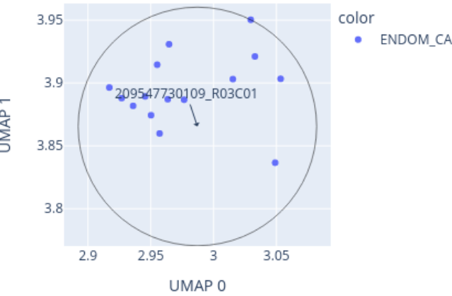
Close-up of UMAP for 209547730109_R03C01 reference: AllIDATv2_20210804_HPAP_Sarc.xlsx (19967 cases), 0 CpGs
