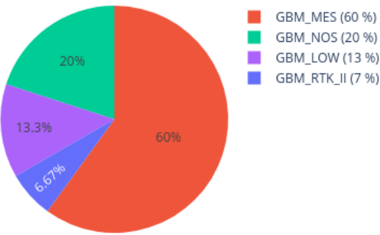
Neighbors in UMAP for 209547730131_R02C01 reference: AllIDATv2_20210804_HPAP_Sarc.xlsx (19967 cases), 0 CpGs
