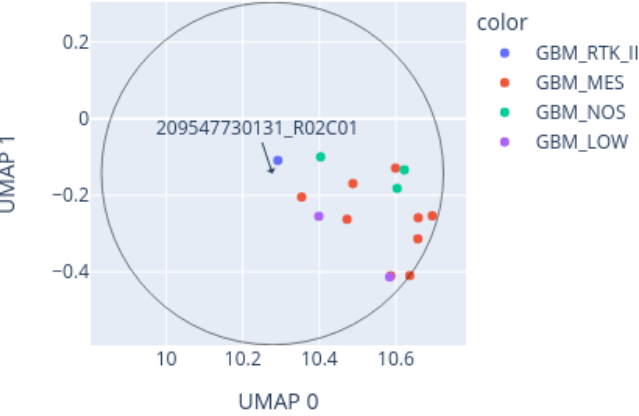
Close-up of UMAP for 209547730131_R02C01 reference: AllIDATv2_20210804_HPAP_Sarc.xlsx (19967 cases), 0 CpGs
