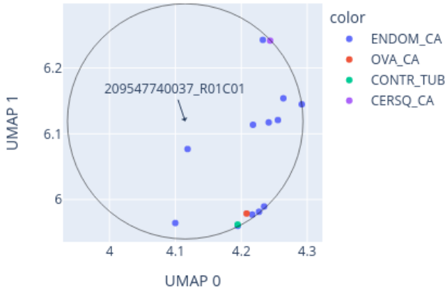
Close-up of UMAP for 209547740037_R01C01 reference: AllIDATv2_20210804_HPAP_Sarc.xlsx (19967 cases), 0 CpGs
