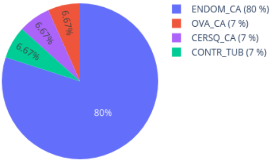
Neighbors in UMAP for 209547740037_R01C01 reference: AllIDATv2_20210804_HPAP_Sarc.xlsx (19967 cases), 0 CpGs
