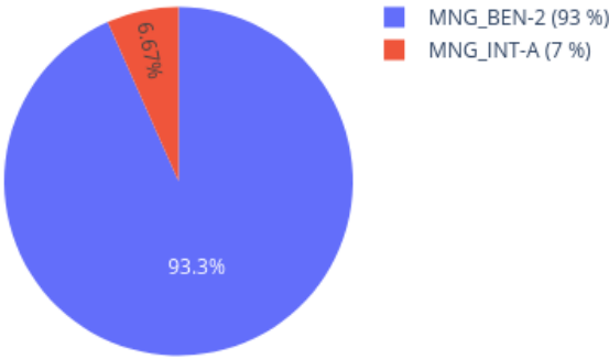
Neighbors in UMAP for 209547740037_R06C01 reference: AllIDATv2_20210804_HPAP_Sarc.xlsx (19967 cases), 0 CpGs
