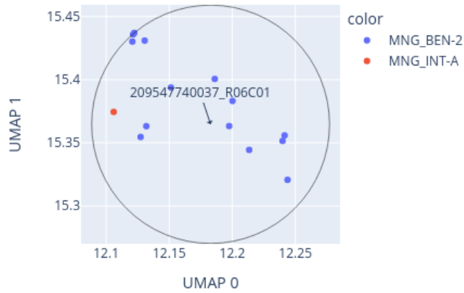
Close-up of UMAP for 209547740037_R06C01 reference: AllIDATv2_20210804_HPAP_Sarc.xlsx (19967 cases), 0 CpGs
