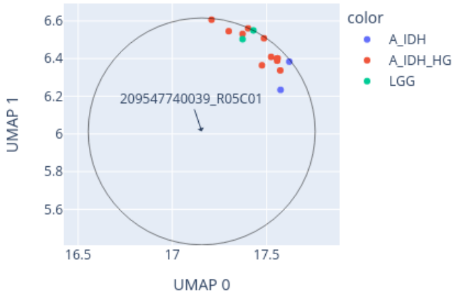
Close-up of UMAP for 209547740039_R05C01 reference: AllIDATv2_20210804_HPAP_Sarc.xlsx (19967 cases), 0 CpGs
