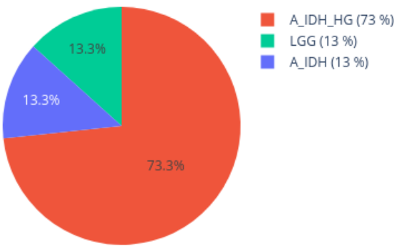
Neighbors in UMAP for 209547740039_R05C01 reference: AllIDATv2_20210804_HPAP_Sarc.xlsx (19967 cases), 0 CpGs
