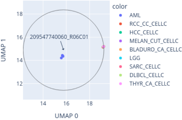
Close-up of UMAP for 209547740060_R06C01 reference: AllIDATv2_20210804_HPAP_Sarc.xlsx (19967 cases), 0 CpGs
