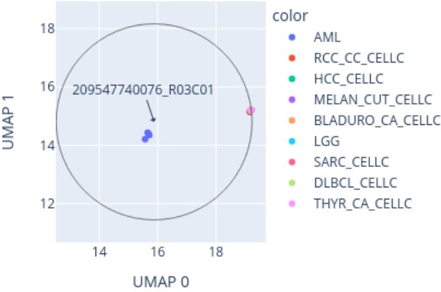
Close-up of UMAP for 209547740076_R03C01 reference: AllIDATv2_20210804_HPAP_Sarc.xlsx (19967 cases), 0 CpGs
