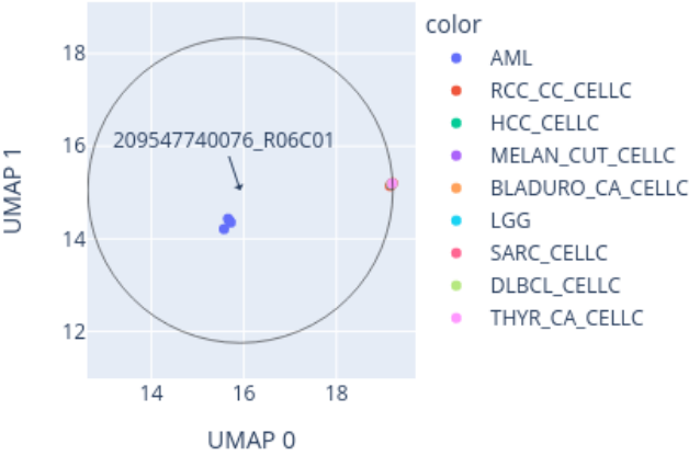
Close-up of UMAP for 209547740076_R06C01 reference: AllIDATv2_20210804_HPAP_Sarc.xlsx (19967 cases), 0 CpGs
