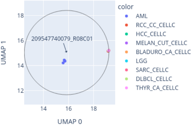
Close-up of UMAP for 209547740079_R08C01 reference: AllIDATv2_20210804_HPAP_Sarc.xlsx (19967 cases), 0 CpGs
