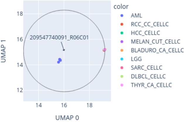
Close-up of UMAP for 209547740091_R06C01 reference: AllIDATv2_20210804_HPAP_Sarc.xlsx (19967 cases), 0 CpGs
