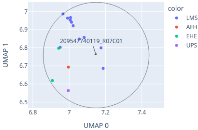
Close-up of UMAP for 209547740119_R07C01 reference: AllIDATv2_20210804_HPAP_Sarc.xlsx (19967 cases), 0 CpGs
