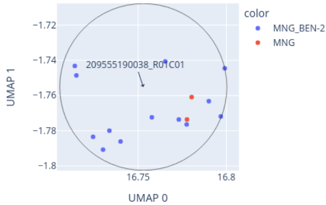
Close-up of UMAP for 209555190038_R01C01 reference: AllIDATv2_20210804_HPAP_Sarc.xlsx (19967 cases), 0 CpGs
