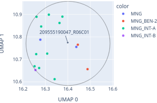
Close-up of UMAP for 209555190047_R06C01 reference: AllIDATv2_20210804_HPAP_Sarc.xlsx (19967 cases), 0 CpGs
