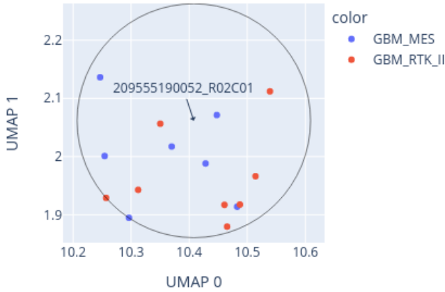
Close-up of UMAP for 209555190052_R02C01 reference: AllIDATv2_20210804_HPAP_Sarc.xlsx (19967 cases), 0 CpGs
