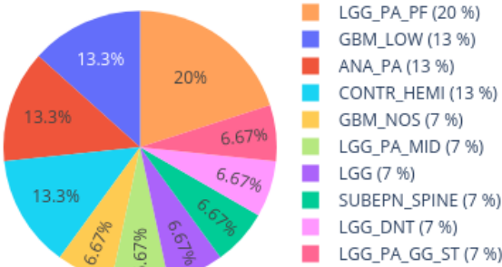
Neighbors in UMAP for 209555190052_R04C01 reference: AllIDATv2_20210804_HPAP_Sarc.xlsx (19967 cases), 0 CpGs
