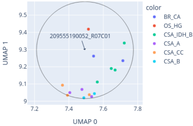
Close-up of UMAP for 209555190052_R07C01 reference: AllIDATv2_20210804_HPAP_Sarc.xlsx (19967 cases), 0 CpGs
