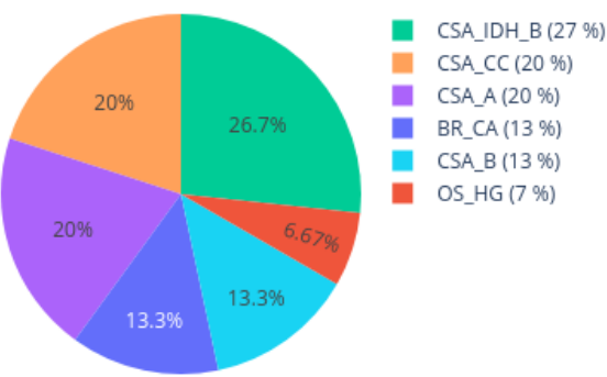
Neighbors in UMAP for 209555190052_R07C01 reference: AllIDATv2_20210804_HPAP_Sarc.xlsx (19967 cases), 0 CpGs
