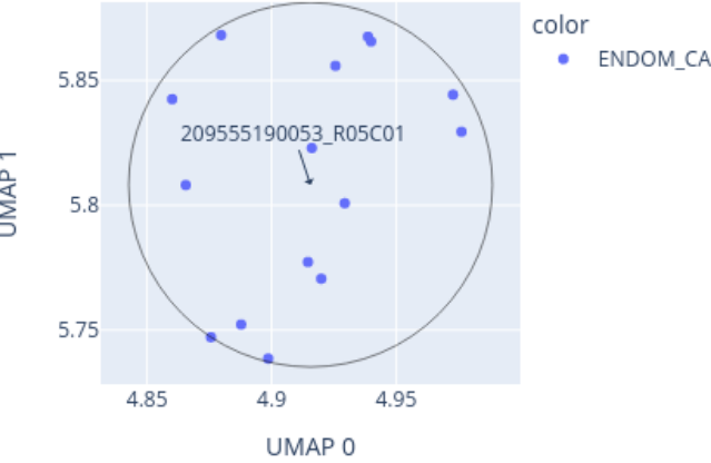
Close-up of UMAP for 209555190053_R05C01 reference: AllIDATv2_20210804_HPAP_Sarc.xlsx (19967 cases), 0 CpGs
