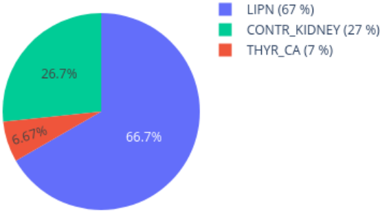
Neighbors in UMAP for 20955530112_R08C01 reference: AllIDATv2_20210804_HPAP_Sarc.xlsx (19967 cases), 0 CpGs
