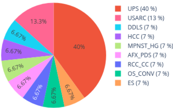
Neighbors in UMAP for 209555540038_R01C01 reference: AllIDATv2_20210804_HPAP_Sarc.xlsx (19967 cases), 0 CpGs
