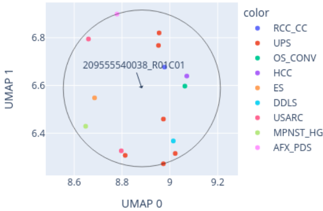
Close-up of UMAP for 209555540038_R01C01 reference: AllIDATv2_20210804_HPAP_Sarc.xlsx (19967 cases), 0 CpGs
