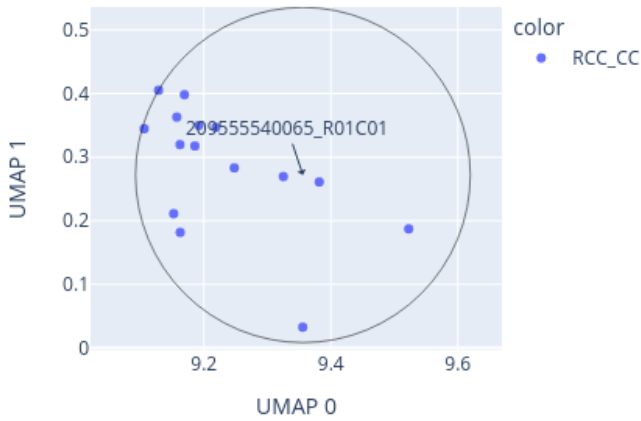
Close-up of UMAP for 209555540065_R01C01 reference: AllIDATv2_20210804_HPAP_Sarc.xlsx (19967 cases), 0 CpGs
