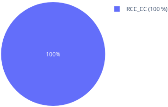
Neighbors in UMAP for 209555540065_R01C01 reference: AllIDATv2_20210804_HPAP_Sarc.xlsx (19967 cases), 0 CpGs
