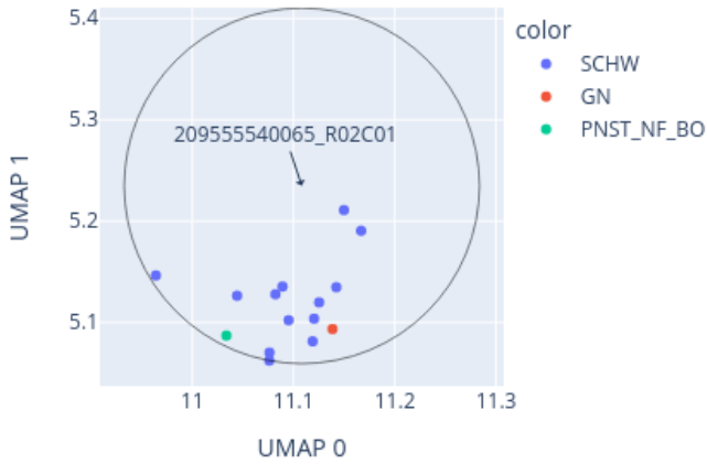
Close-up of UMAP for 209555540065_R02C01 reference: AllIDATv2_20210804_HPAP_Sarc.xlsx (19967 cases), 0 CpGs
