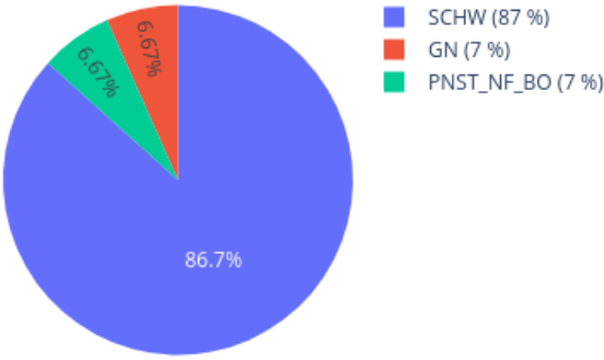
Neighbors in UMAP for 209555540065_R02C01 reference: AllIDATv2_20210804_HPAP_Sarc.xlsx (19967 cases), 0 CpGs
