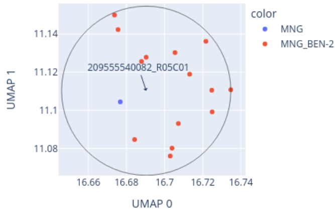
Close-up of UMAP for 209555540082_R05C01 reference: AllIDATv2_20210804_HPAP_Sarc.xlsx (19967 cases), 0 CpGs
