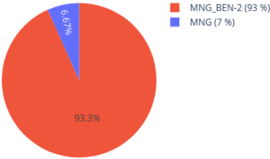
Neighbors in UMAP for 209555540082_R05C01 reference: AllIDATv2_20210804_HPAP_Sarc.xlsx (19967 cases), 0 CpGs
