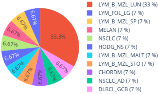
Neighbors in UMAP for 209555540095_R06C01 reference: AllIDATv2_20210804_HPAP_Sarc.xlsx (19967 cases), 0 CpGs
