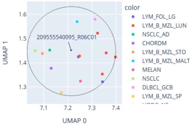
Close-up of UMAP for 209555540095_R06C01 reference: AllIDATv2_20210804_HPAP_Sarc.xlsx (19967 cases), 0 CpGs
